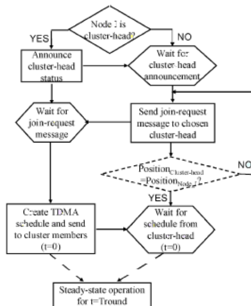
Figure 4. Flowchart of O-LEACH algorithm [1]
