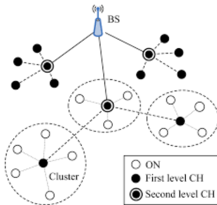
Figure 2. Cluster based wireless sensor network.
